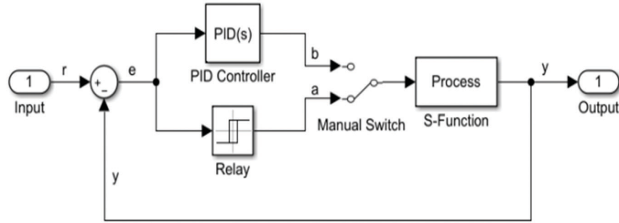
Figure 6. Schematic diagram for the Pid controller.
