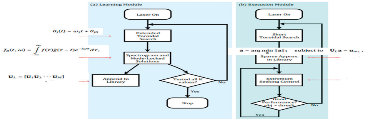
Figure 4. Global searching algorithm.
