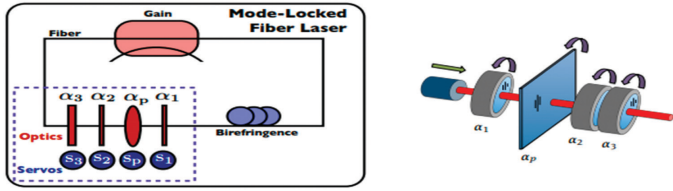
Figure 1. Schematic diagram for the mode-locked fiber laser, ADAPTED [12].
