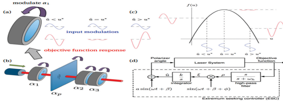
Figure 3. Schematic diagram; (a) samples of the polarization angle; (b) modelling of multi-loop gain; (c) input-output curves; (d) proposed control system.
