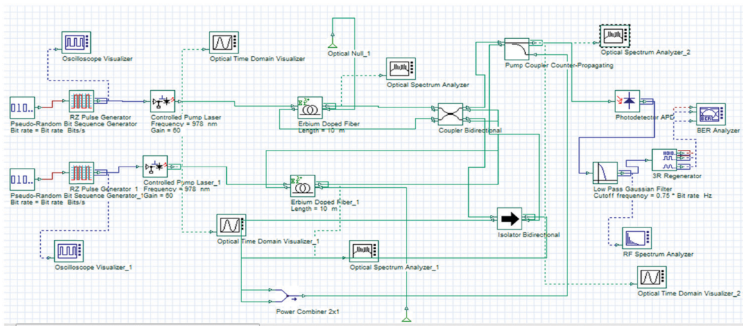
Figure 5. Simulation setup of the double laser system.
