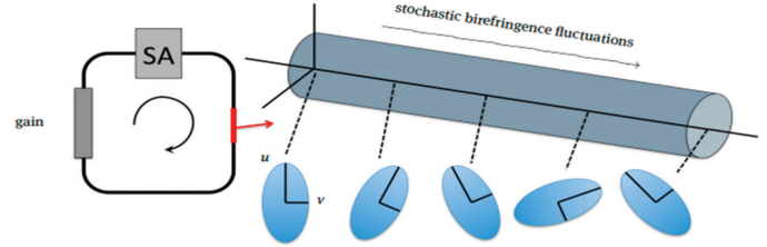
Figure 2. Schematic diagram for the polarization angle effects, adapted from [13].
