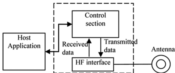
Figure 2. The components of an RFID reader.
