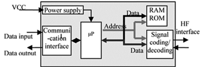
Figure 3. The components of the control section of the RFID reader.
