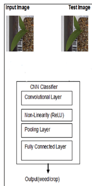
Figure 1. Weed detection architecture.
