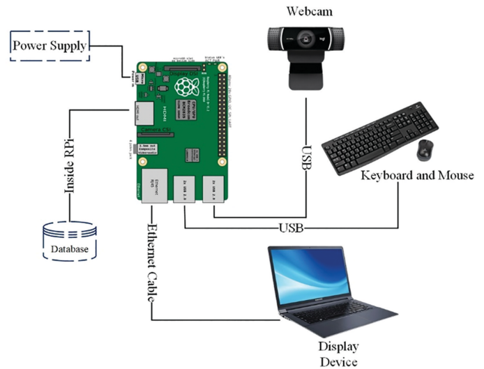
Figure 5. System design of Pasurmarti et al. [6].
