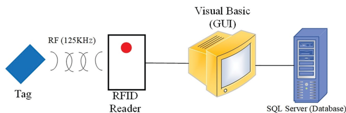
Figure 7. System Design of Arulogun et al. [8].
